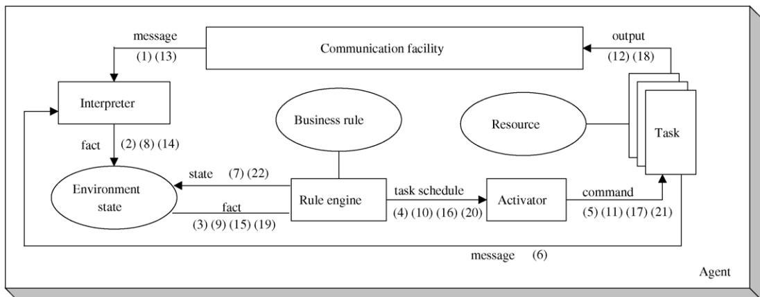
Fig. 5. Operation of the cognitive agent.
